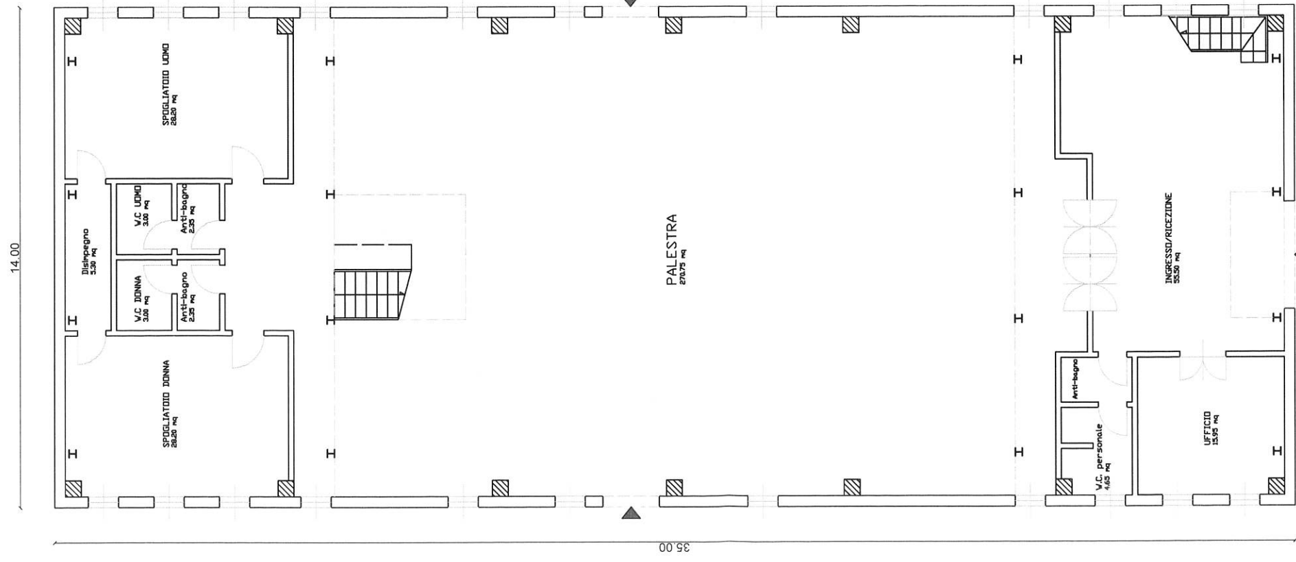
PIANO TERRA
